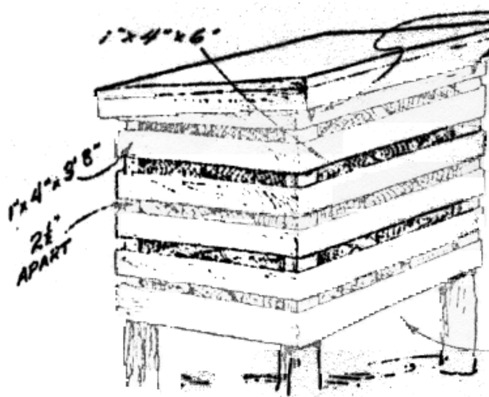
HERE'S THE "STANDARD" FEEDING SHELTER FOR GAME. WHEN BUILT ON UNFROZEN GROUND IT CAN BE SUPPORTED BY FORMED STAKES INSTEAD OF TREES. CAN BE COVERED WITH CORN STALKS, BARK, OR BRUSH & LEAVES.
